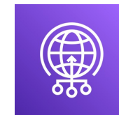
Global Accelerator
