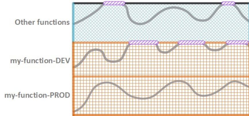
Reserved Concurrency
