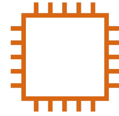
EC2 Instance
